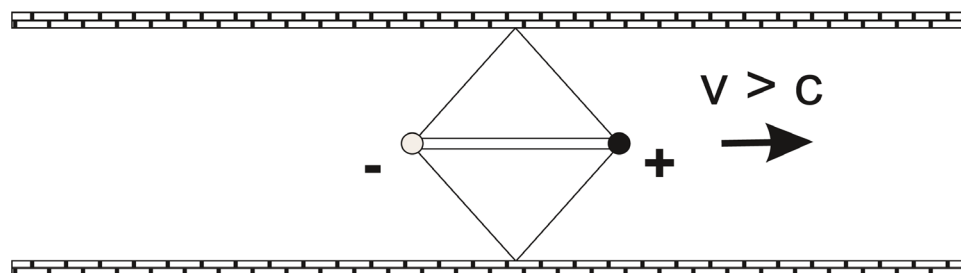
Figure 1. Inferred (proposed) superluminal electromagnetic wave structure that is generated by a combination of two massless particles with equal charge but different signs moving at a superluminal speed in a tunnel.
