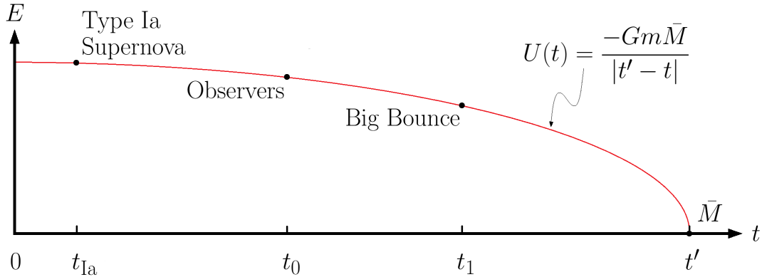
Figure 22: This figure depicts the Newtonian mechanism for MCM dark energy mostly as it appeared in [31]. t_{1a} is the proper time of a high redshift supernova in the dark energy survey. Such supernovae live on the past light cone of an observer with proper time t_0 . The upcoming bounce lies at t_1 . t' is the temporal midpoint of the cycle of cosmology beyond the bounce and \bar{M} is a point mass representing the universe in the cycle beyond the bounce. The energy curve assumes that every slice of constant proper time in our present cycle of cosmology has the same mass m so the energy between \bar{M} and the slices of constant proper time at t_{1a} or t_0 differs only in the timelike separation |t' - t| . Observers in an inertial frame at t_0 will see objects at t_{1a} appear to recede under acceleration because t_0 is deeper into \bar{M} 's gravitational well.
