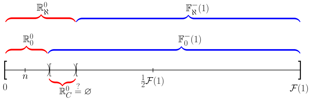
Figure 2: This figure ( not to scale! ) shows the neighborhood of the origin \mathbb{R}_\mathbb{N}^0 , the substructure of that neighborhood, and the associated structure from the Cantor-like sets. \mathbb{F}^- refers to the subset of \mathbb{F} which is less than or equal to \mathcal{F}(1) = \mathcal{F}_0 .
