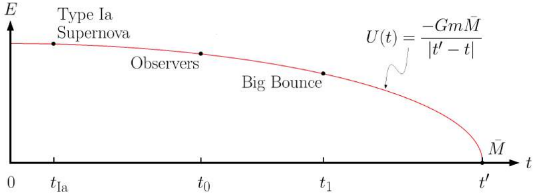
Figure 22: This figure depicts the Newtonian mechanism for MCM dark energy, mostly as it appeared in [31]. t_{1a} is the proper time of a high redshift supernova in the dark energy survey. Such supernovae live on the past light cone of an observer with proper time t_0 . The upcoming bounce lies at t_1 . t' is the temporal midpoint of the cycle of cosmology beyond the bounce and \bar{M} is a point mass representing the universe in the cycle beyond the bounce. The energy curve assumes that every slice of constant proper time in our present cycle of cosmology has the same mass m so the energy between \bar{M} and the slices of constant proper time at t_{1a} or t_0 differs only in the timelike separation |t' - t| . Observers in an inertial frame at t_0 will see objects at t_{1a} appear to recede under acceleration because t_0 is deeper into \bar{M} 's gravitational well.
