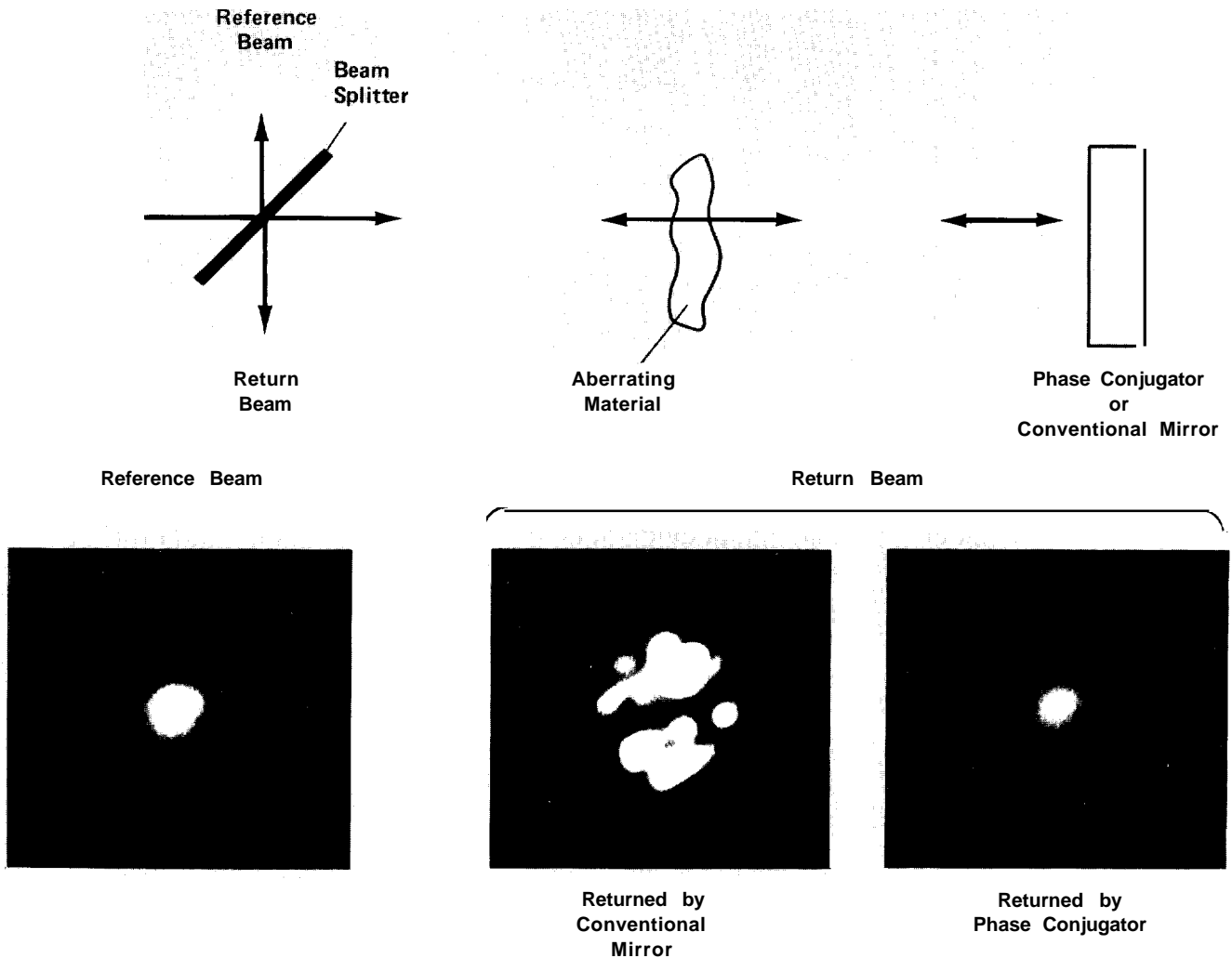
Fig. 3. Experimental demonstration of phase-conjugate reflection. An undistorted laser beam (left photograph) is double passed through an aberrating material. Conventional reflection for the return trip results in a highly distorted beam
