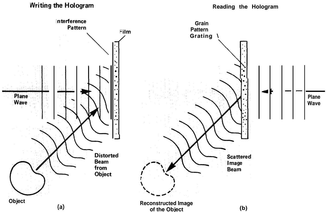
Fig. 6. Conventional holography consists of two distinct "write" and "read" steps. (a) First, the film is exposed to the interference pattern formed by an undistorted reference beam with a distorted beam reflected off the object. The result, after development of the film, is the hologram, a grain pattern in the emulsion. (b) A second undistorted reference beam, here
