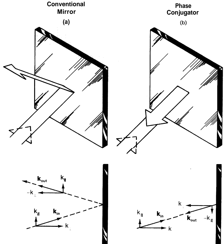
Fig. 1. (a) A conventional mirror reflects light by inverting only the normal component k_{\perp} of the beam's propagation vector \mathbf{k} . This process leads to the law that the angle of incidence equals the angle of reflection and allows the direction of the reflected beam to be altered by changing the tilt of the mirror. (b) A phase conjugator reflects light by inverting all components so that the propagation vector changes sign ( \mathbf{k}_{out} = -\mathbf{k}_{in} ). In this case, regardless of the tilt of the mirror, the reflected light exactly retraces the path of the incoming beam.
