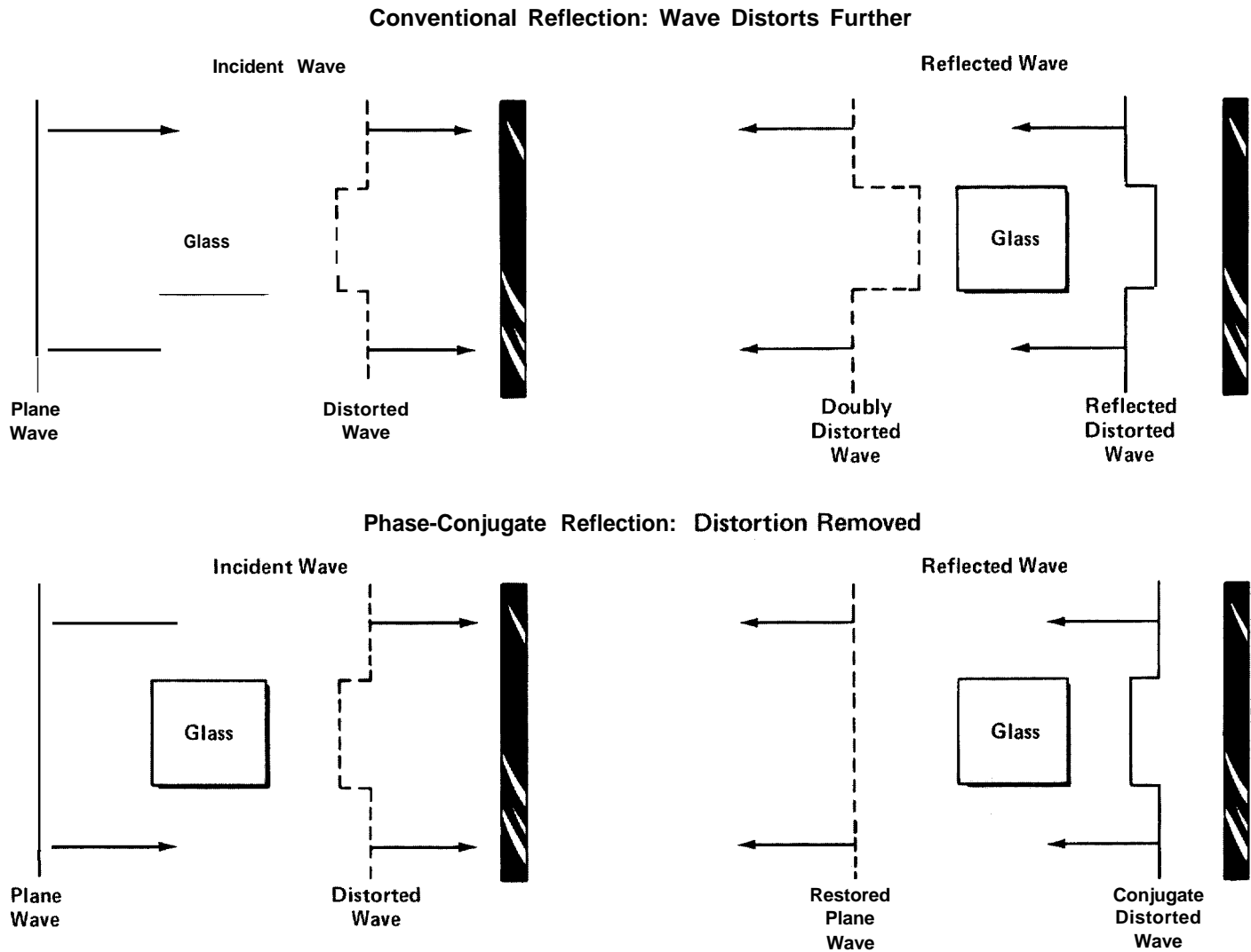
Fig. 2. Phase distortion with conventional and phase-conjugate reflection. In both cases the incoming plane wave (left side) encounters a block of glass, and a distorted wave is formed because the glass, with a different refractive index, retards the phase of the wave's central region. Conventional reflection (top right) retains this lag in phase so that the return trip through
