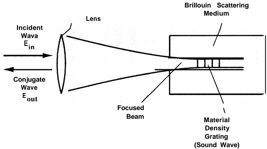
Fig. 8. Backward stimulated Brillouin scattering. The incoming field E_{in} interacts with an acoustic wave to produce a backward scattered wave E_{out} and also interacts with E_{out} (through the medium) to produce an acoustic wave. The two processes positively reinforce each other only when E_{out} is the phase conjugate of E_{in} .
