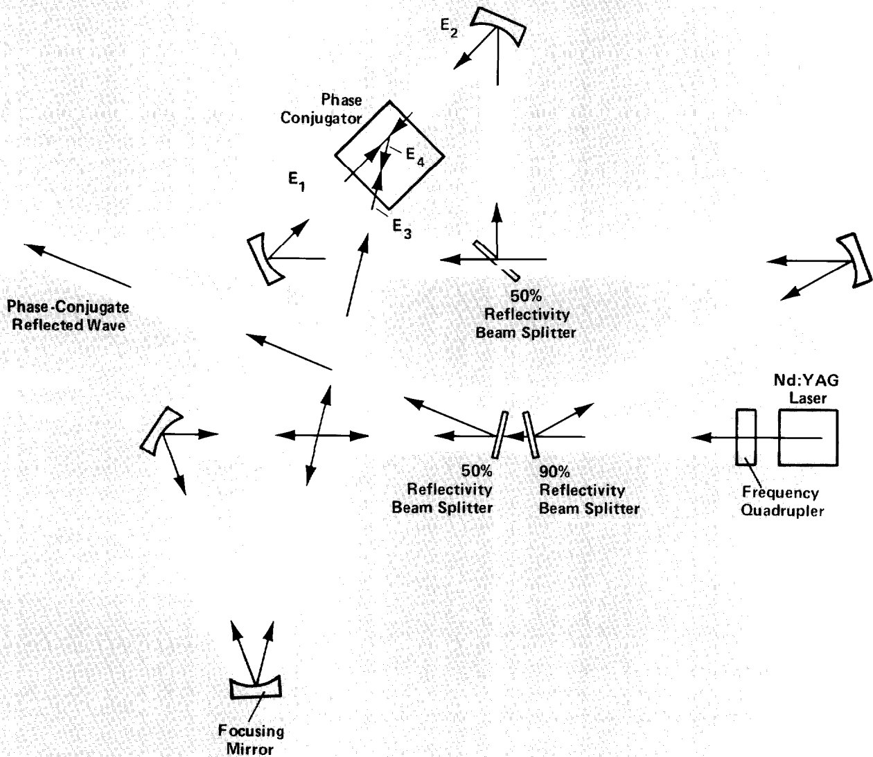
Fig. 12. Degenerate four-wave mixing in the ultraviolet. The frequency-quadrupled output (266-nanometer wavelength) of a Nd:YAG laser is split so that 90 per cent of the beam is directed to the phase conjugator as two counterpropagating
