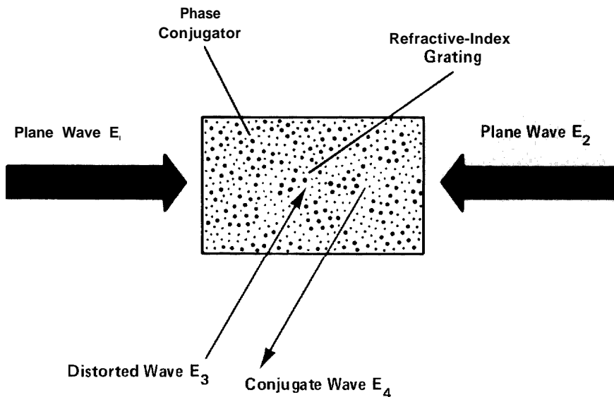
Fig. 7. In degenerate four-wave mixing the write and read steps of holography take place simultaneously. Interference of the intense plane wave E_1 and the distorted wave E_3 , generates a refractive-index grating in the nonlinear optical material of the phase conjugator. The intense counterpropagating plane wave E_2 immediately scatters off this grating to form the reflected wave E_4 , that is the phase conjugate of E_3 . Because the roles of E_1 and E_2 can be exchanged, a second wave, indistinguishable from E_1 , is also produced. The intensity of the reflected wave is a function of the three incident fields ( E_1 , E_2 , and E_3 ) and of the material properties of the phase conjugator (such as the magnitude of its nonlinear optical effect).
