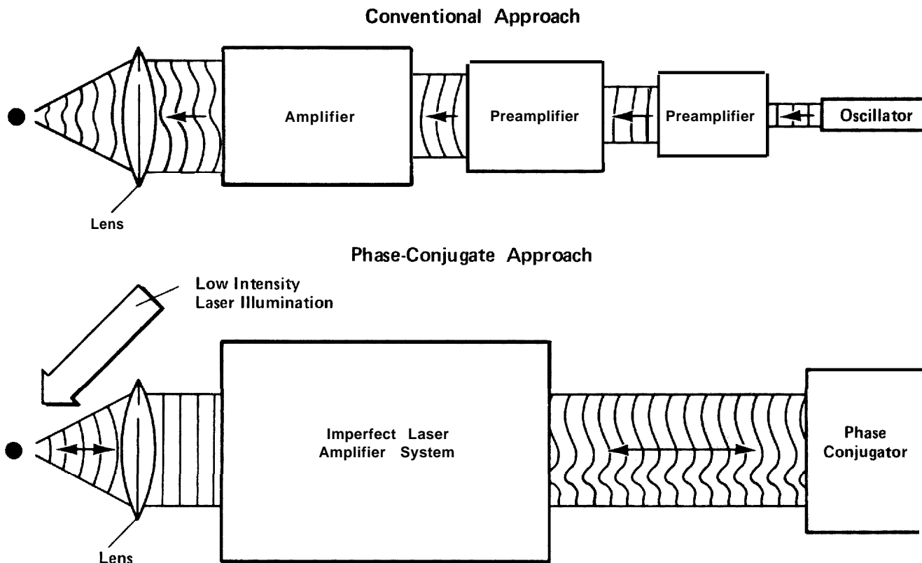
Fig. 15. Laser fusion systems. The conventional system (top) uses a long chain of laser amplifiers that may gradually introduce distortions in the beam arriving at the fusion target. In the phase-conjugate laser fusion system (bottom), a spatially broad, low-intensity laser illuminates the target. A small fraction of this illumination is reflected off the fusion target into the solid angle of the focusing optics and is
