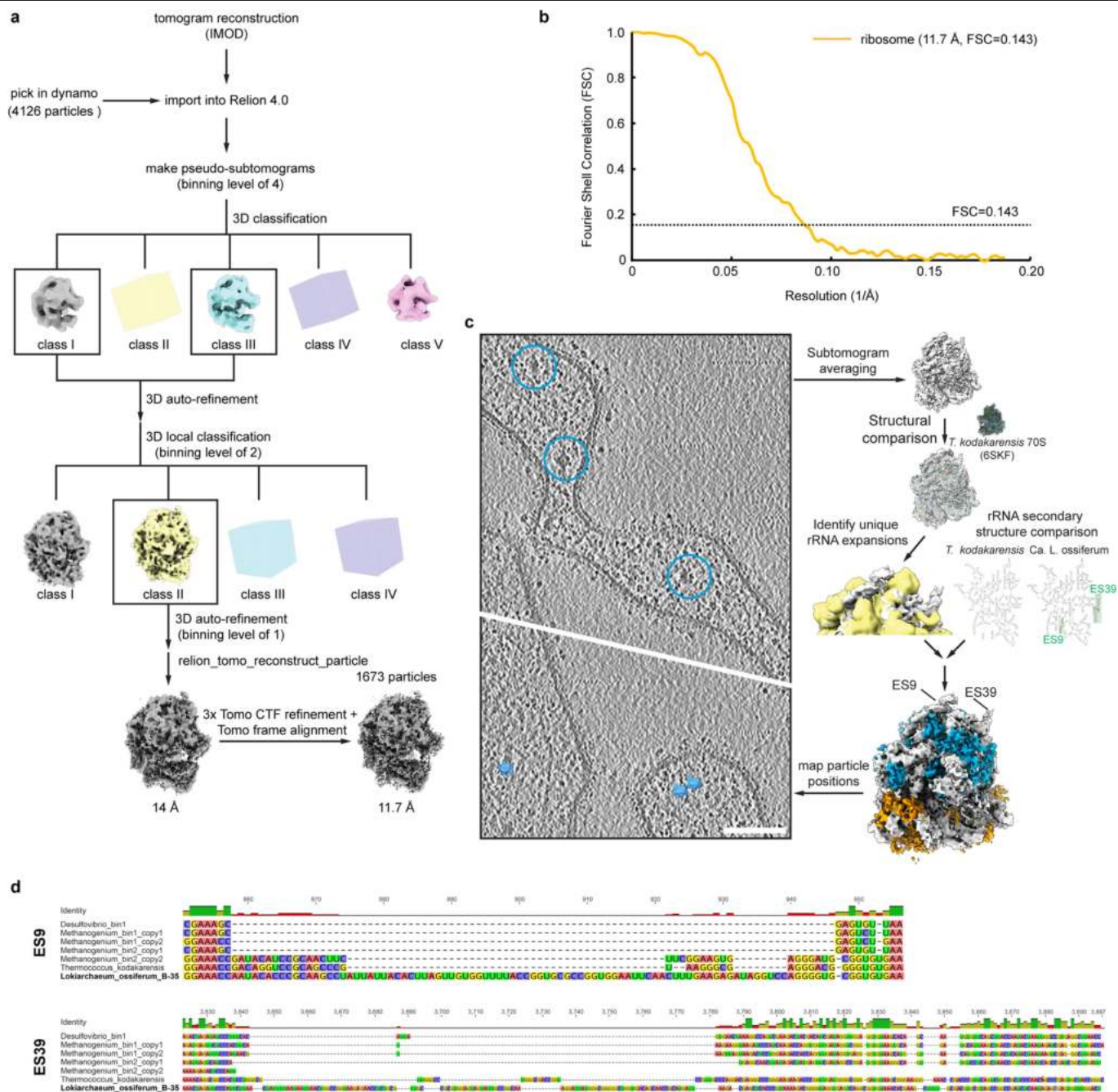
Extended Data Fig. 6 | Sub-tomogram averaging of the ribosome and identification of rRNA expansion segments. a. Flowchart for the sub-tomogram averaging strategy of the ribosome. For details see Methods. b. Gold-standard FSC curve of the sub-tomogram average. c. Scheme of the ribosome identification workflow. For details see Fig. 3 and Methods. d. Multiple sequence alignment of expansion segments (ESs) 9 and 39 of the
